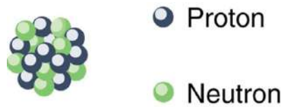
FIGURE 31.11 A model of the nucleus.
