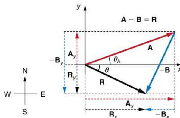
FIGURE 3.33 The subtraction of the two vectors shown in Figure 3.28 . The components of -\mathbf{B} are the negatives of the components of \mathbf{B} . The method of subtraction is the same as that for addition.
