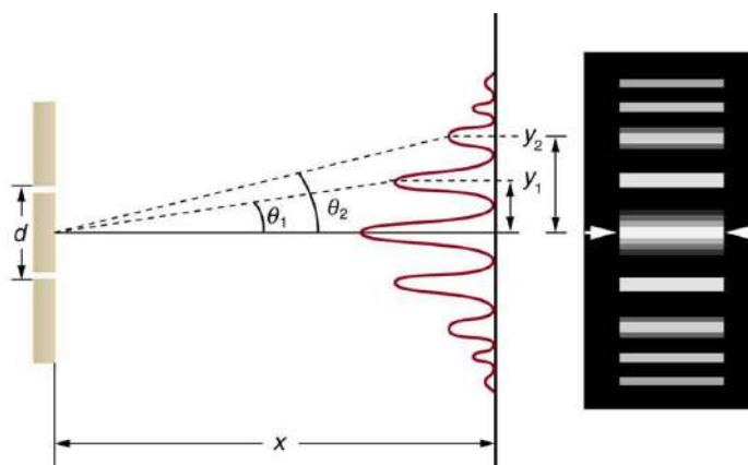
FIGURE 27.15 The interference pattern for a double slit has an intensity that falls off with angle. The photograph shows multiple bright and dark lines, or fringes, formed by light passing through a double slit.
