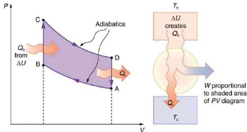
FIGURE 15.18 PV diagram for a simplified Otto cycle, analogous to that employed in an internal combustion engine. Point A corresponds to the start of the compression stroke of an internal combustion engine. Paths AB and CD are adiabatic and correspond to the compression and power strokes of an internal combustion engine, respectively. Paths BC and DA are isochoric and accomplish similar results to the ignition and exhaust-intake portions, respectively, of the internal combustion engine's cycle. Work is done on the gas along path AB, but more work is done by the gas along path CD, so that there is a net work output.
