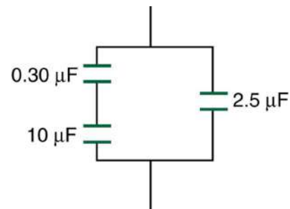
FIGURE 19.32 A combination of series and parallel connections of capacitors.
