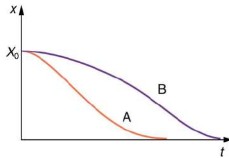
FIGURE 16.21 Displacement versus time for a critically damped harmonic oscillator (A) and an overdamped harmonic oscillator (B). The critically damped oscillator returns to equilibrium at X = 0 in the smallest time possible without overshooting.
