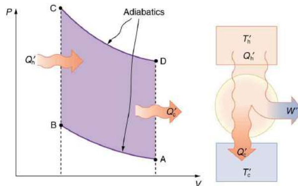
FIGURE 15.19 This Otto cycle produces a greater work output than the one in Figure 15.18 , because the starting temperature of path CD is higher and the starting temperature of path AB is lower. The area inside the loop is greater, corresponding to greater net work output.
