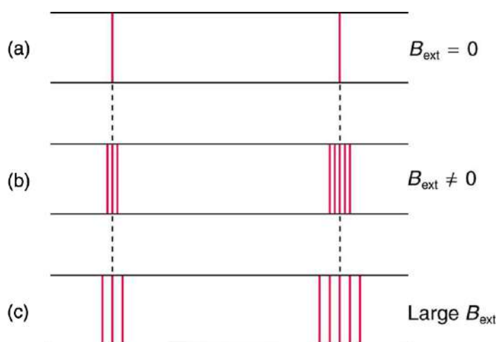
FIGURE 30.47 The Zeeman effect is the splitting of spectral lines when a magnetic field is applied. The number of lines formed varies, but the spread is proportional to the strength of the applied field. (a) Two spectral lines with no external magnetic field. (b) The lines split when the field is applied. (c) The splitting is greater when a stronger field is applied.
