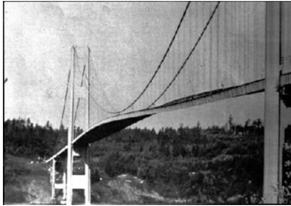
FIGURE 16.26 In 1940, the Tacoma Narrows Bridge in Washington state collapsed. Heavy cross winds drove the bridge into oscillations at its resonant frequency. Damping decreased when support cables broke loose and started to slip over the towers, allowing increasingly greater amplitudes until the structure failed (credit: PRI's Studio 360 , via Flickr)
